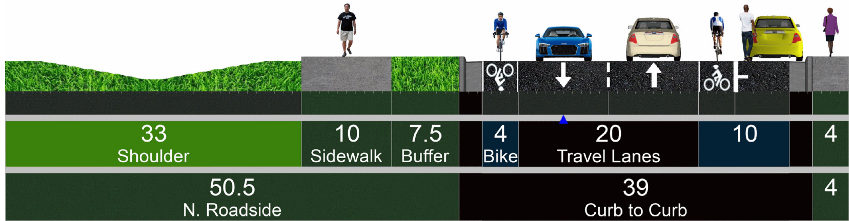
Existing School Access to Colorado Boulevard Cross Section Street Widens at Intersections to Create Left Turn Lanes
