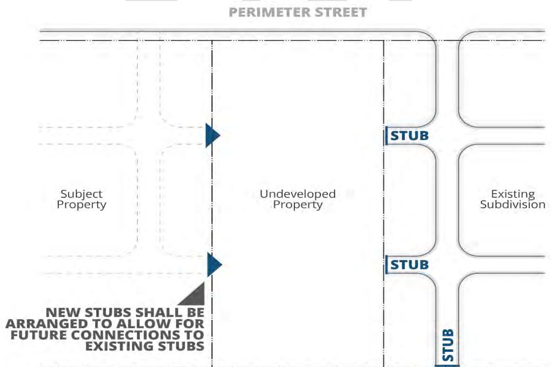
Figure 18-637.4. Street stubs, aligned with nearby street stubs.
