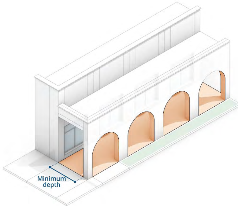
Figure 18-550.6. Example of a pedestrian arcade.
