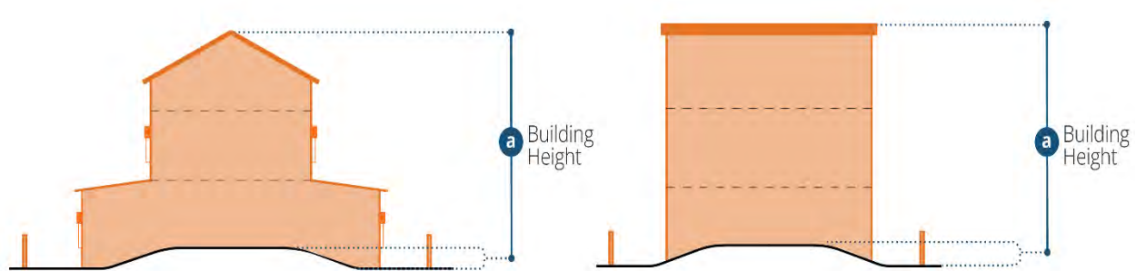
Figure 18-141.1. Building height measurement.
