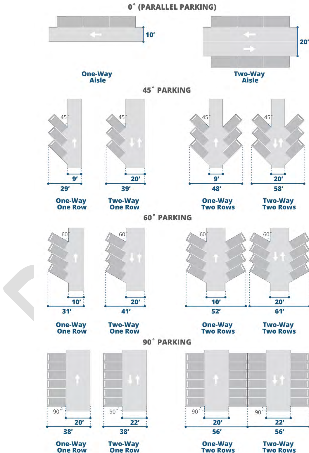
Figure 18-659.3. 10-foot wide spaces.
