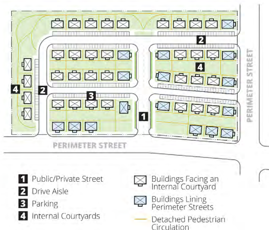
Figure 18-304.1. Large Cottage Housing development example.
