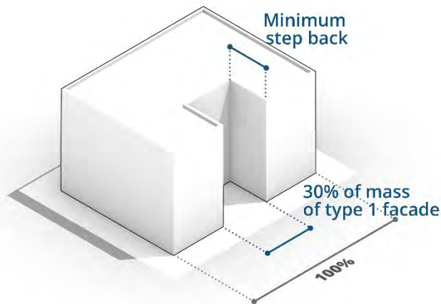
Figure 18-540.3. Example of a “C” or “U” shaped building.
