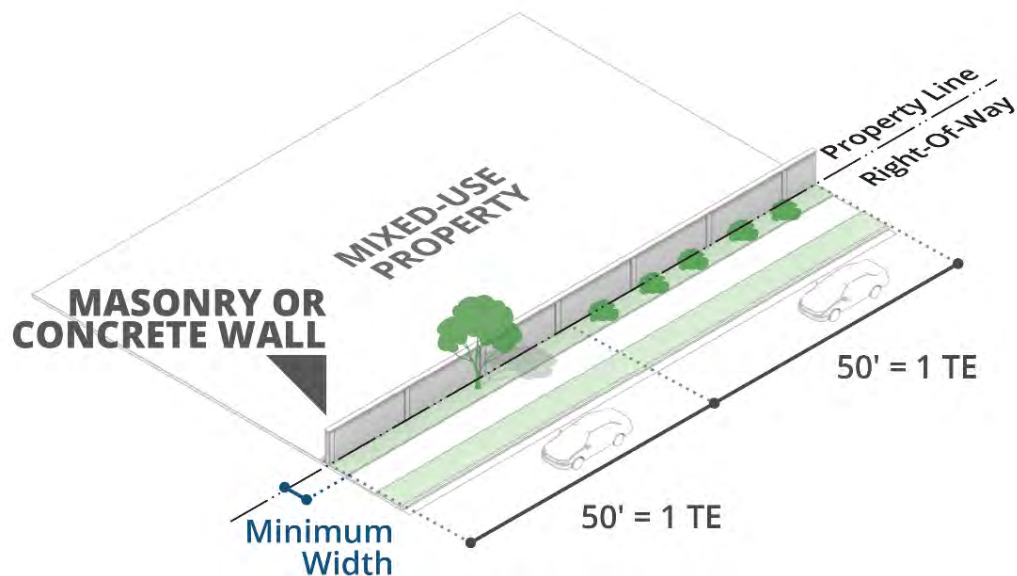
Figure 18-599.9. Mixed-use and nonresidential street buffer requirements – Minor Arterial/Collector Option 1.
