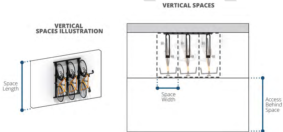
Figure 18-662.4. Short-term bicycle parking – vertical spaces.
