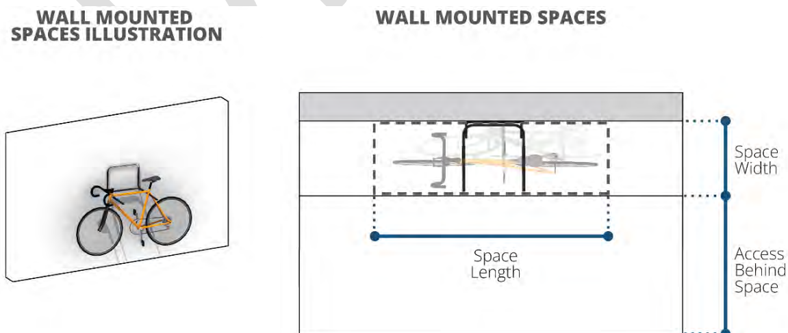
Figure 18-662.3. Short-term bicycle parking – wall mounted spaces.
