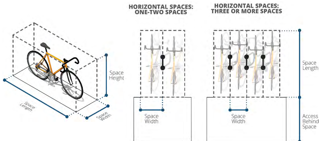
Figure 18-662.2. Short-term bicycle parking – horizontal spaces.
