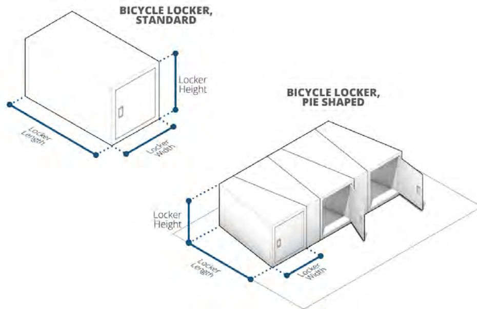
Figure 18-662.5. Short-term bicycle parking – bike locker spaces.
