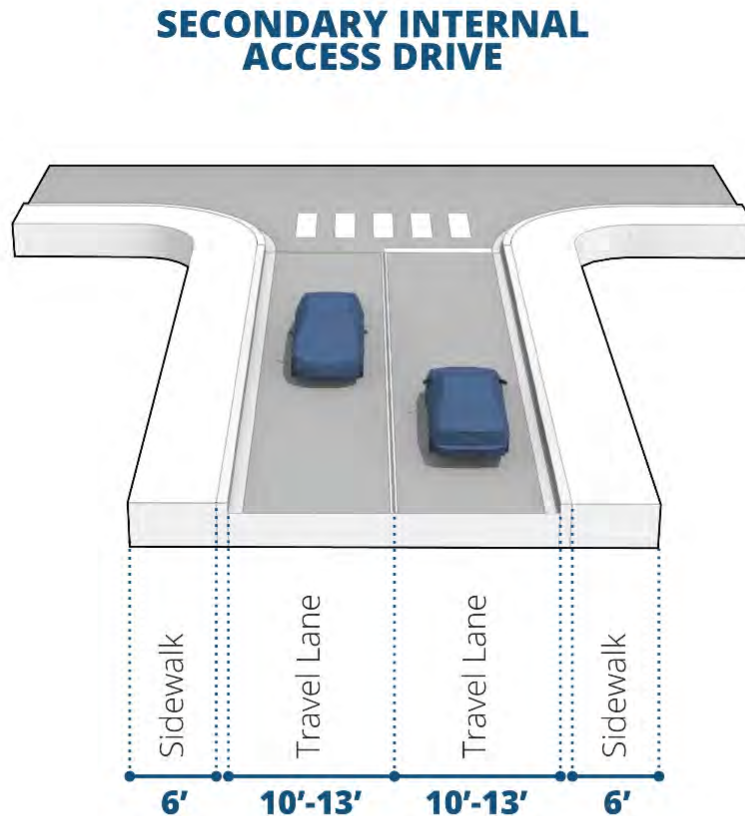
Figure 18-660.2. Secondary internal access drive.
