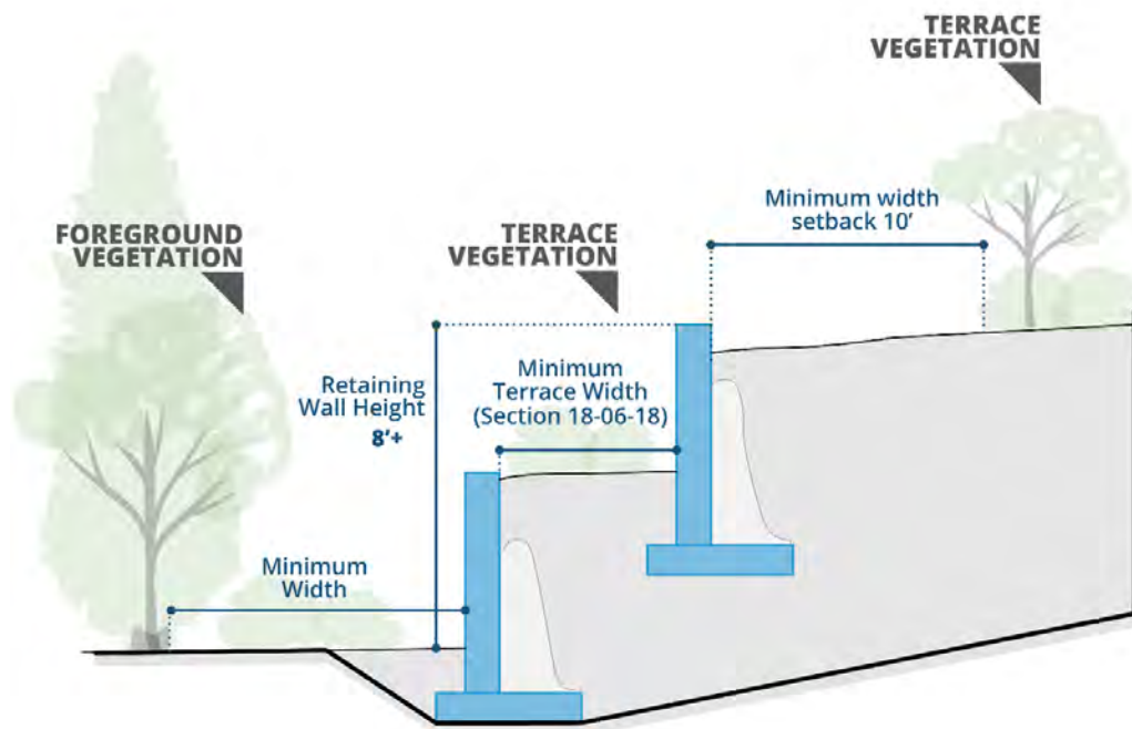
Figure 18-605.2. Retaining wall and wall system landscape, 8+ feet.
