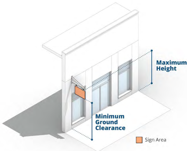
Figure 18-739.1. Projecting signs.
