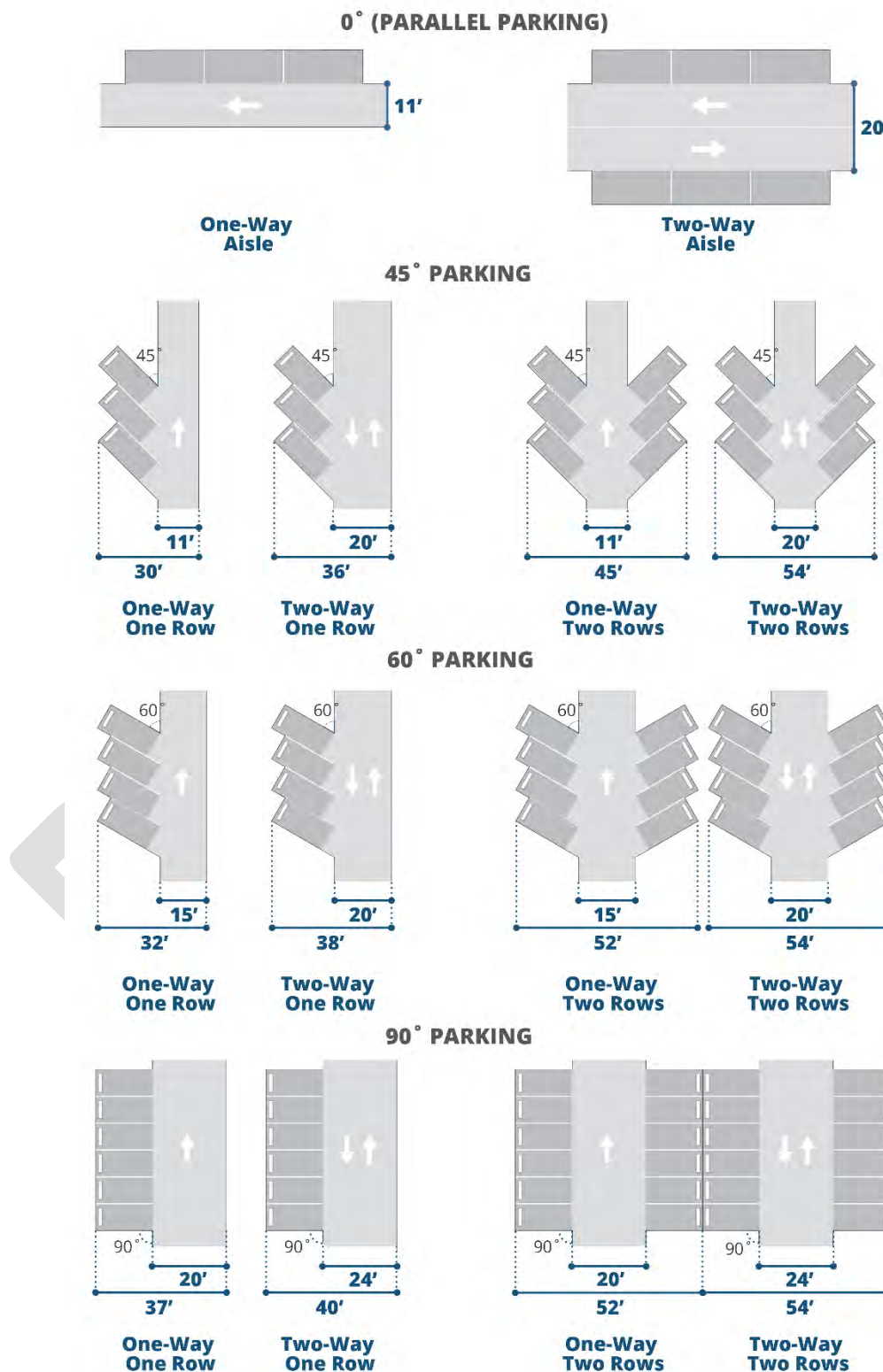
Figure 18-659.1. 8.5-foot wide spaces.
