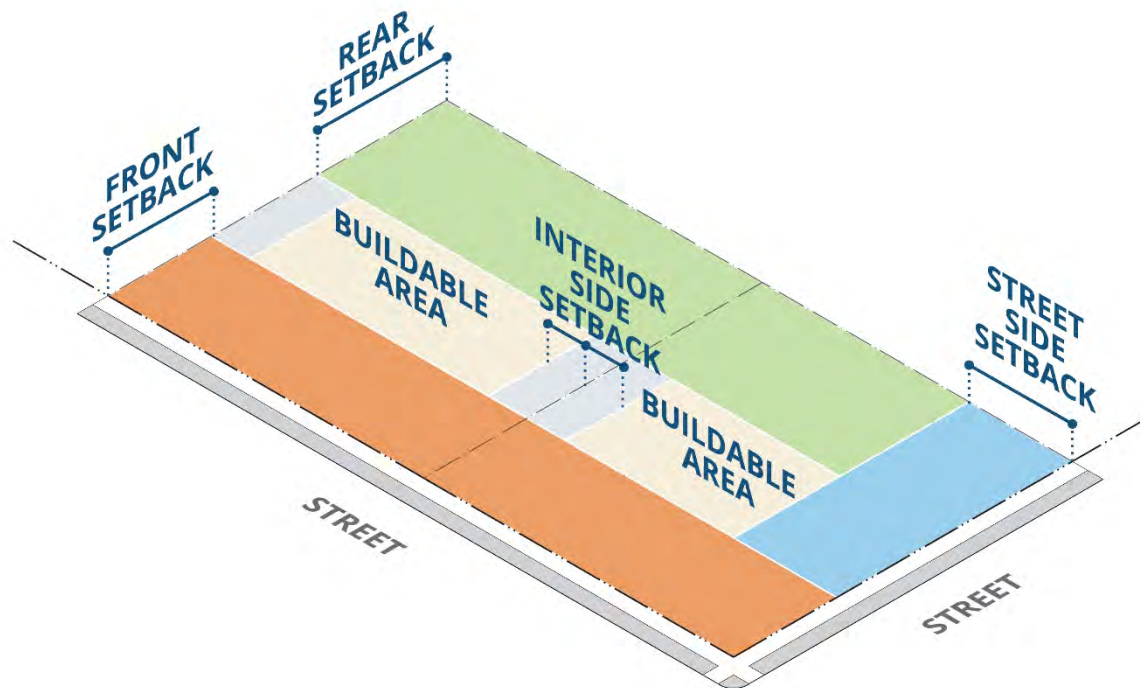
Figure 18-140.1. Yard setback depth measurement.
