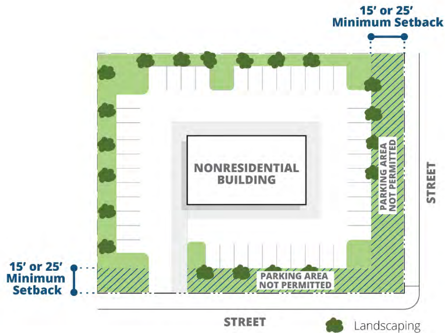
Figure 18-648.5. Parking locations in the RC, BP, and CI Zone Districts.
