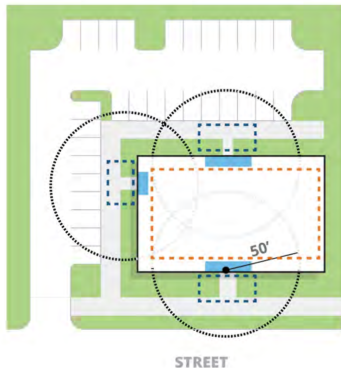
Figure 18-662.6. Short-term and long-term bicycle parking locational standards.
