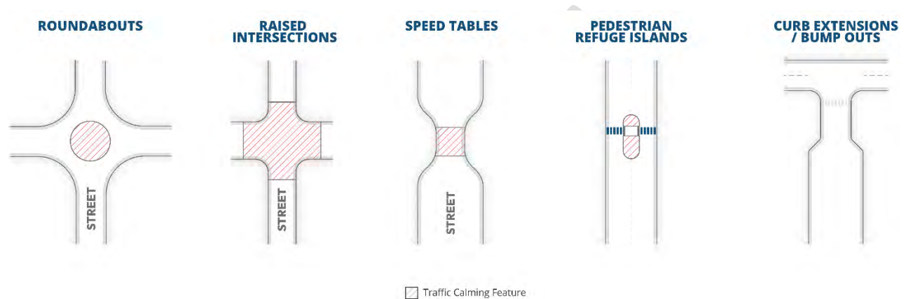
Figure 18-638.1. Traffic calming.
