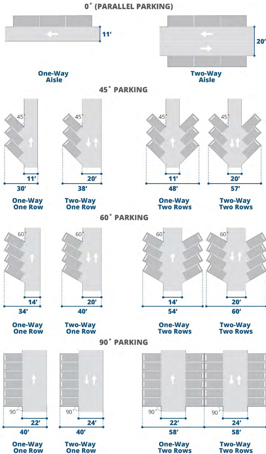
Figure 18-659.2. 9-foot wide spaces.
