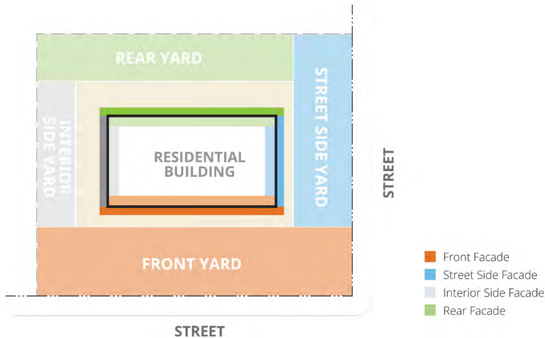
Figure 18-530.1. Residential façade types.
