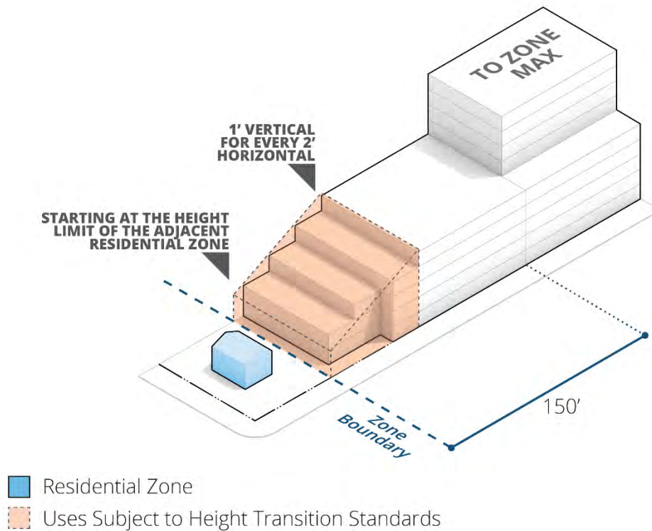
Figure 18-142.2. Height transition standards, when separated by a street.
