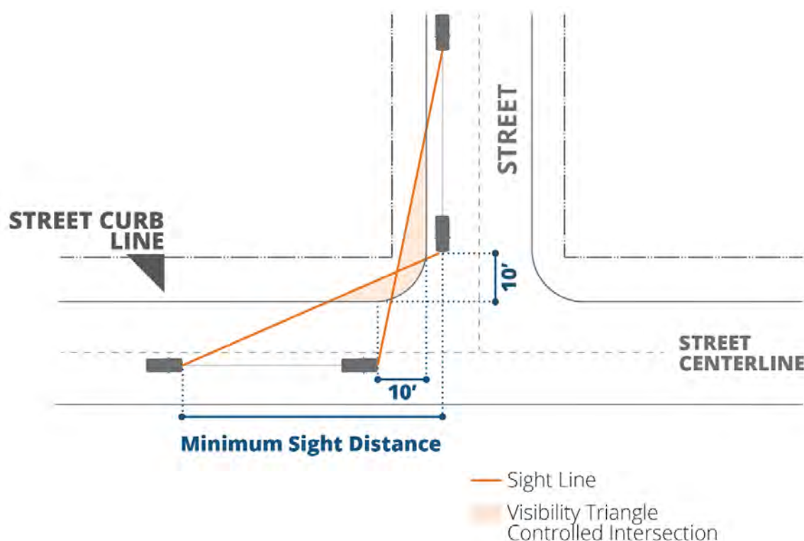
Figure 18-508.1. Visibility triangle for street intersections.
