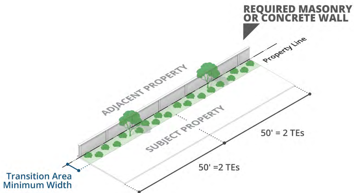
Figure 18-600.4. Transition landscape buffer Option 4.
