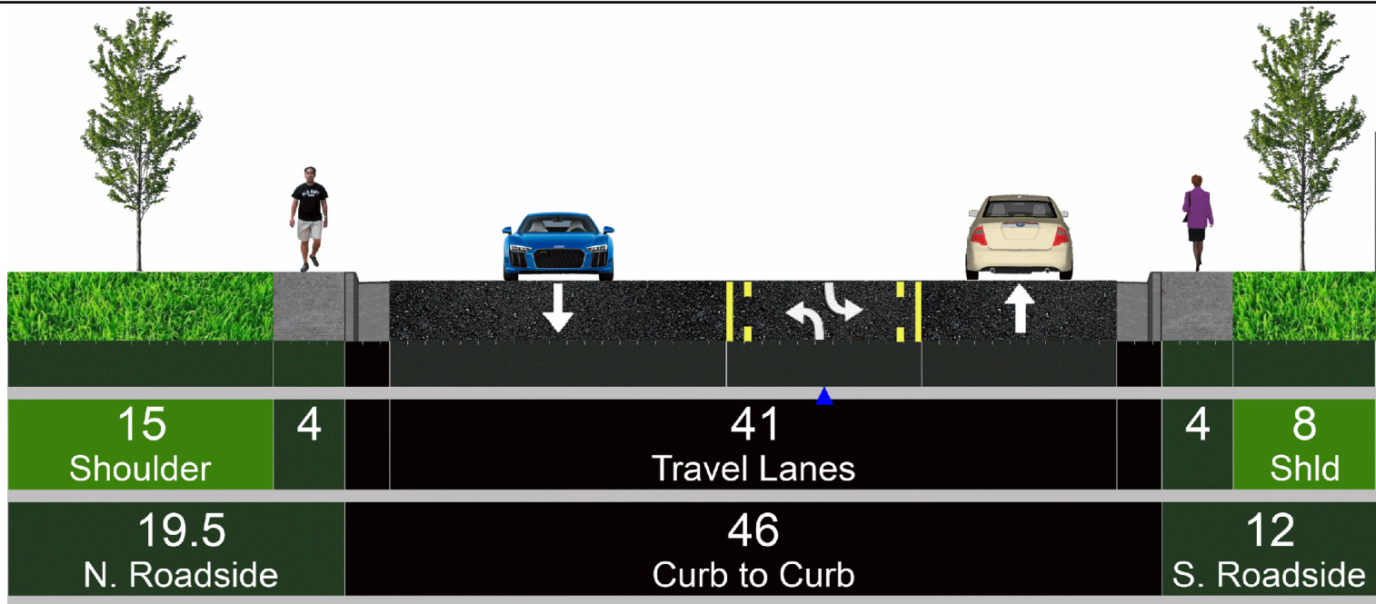
Existing Fillmore St to Steele St Cross Section Landscaping on North Side Extends to Tennis Courts
