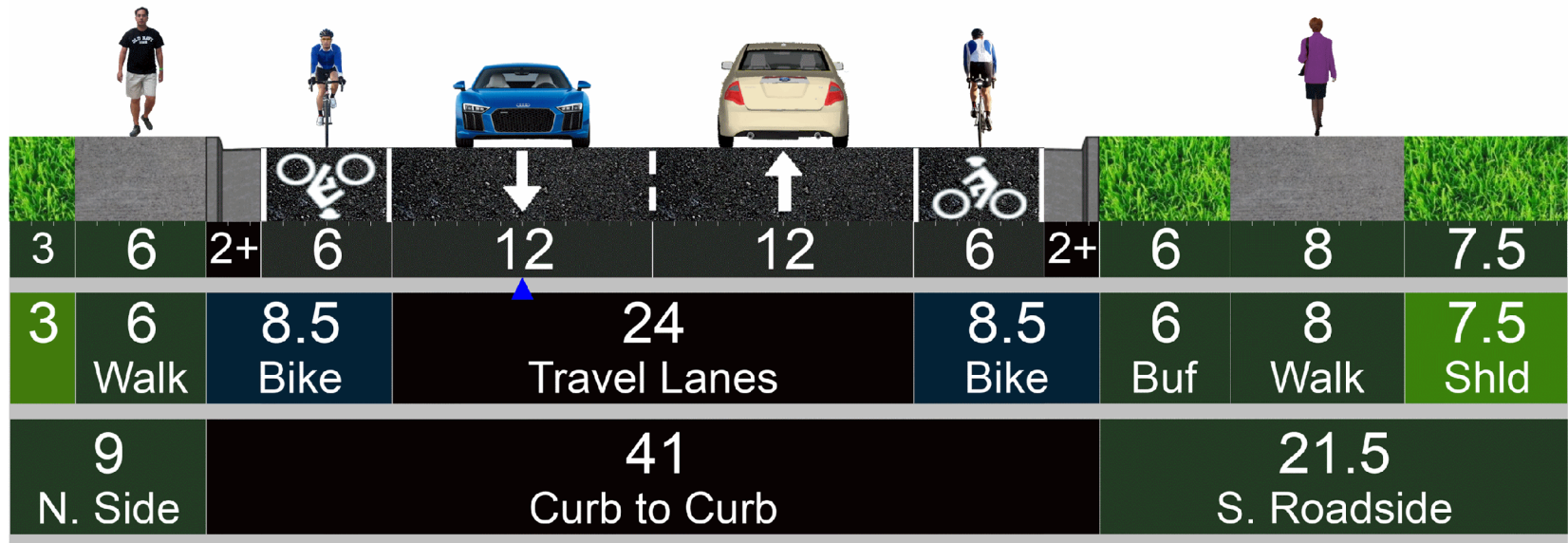
Proposed First St to York St Cross Section Bicycle Lanes End at the York Street Roundabout
