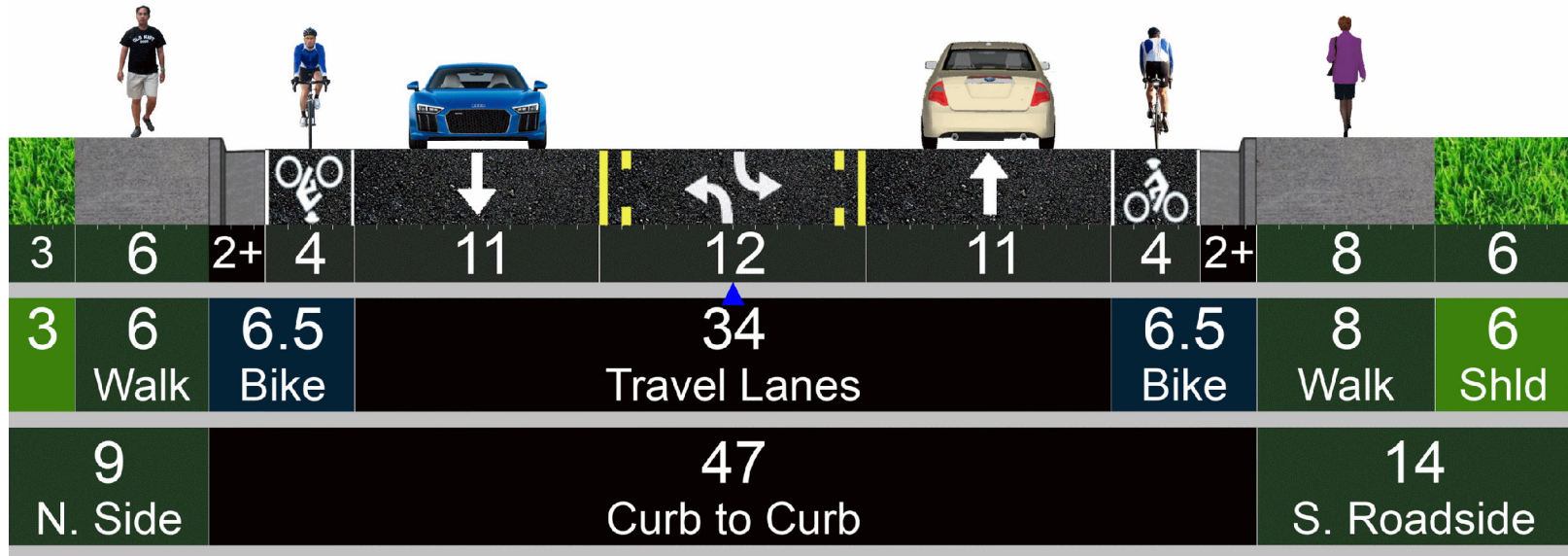
Existing First St to York St Cross Section
