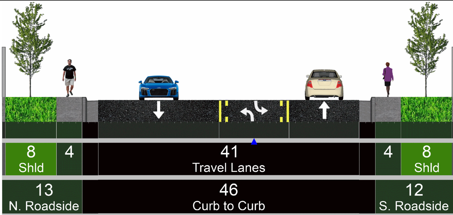
Existing Josephine St to Fillmore St Cross Section
