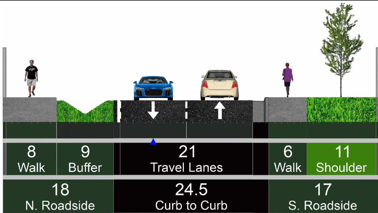
Existing Madison Ct to Monroe Dr Cross Section Street Widens at the Monroe Drive Roundabout to Create Median
