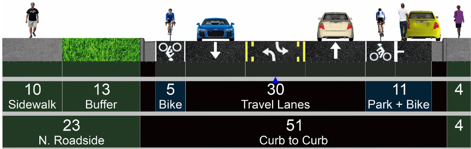
Existing Monroe Dr to School Access Cross Section
