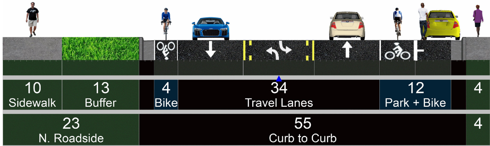
Proposed Monroe Dr to School Access Cross Section
