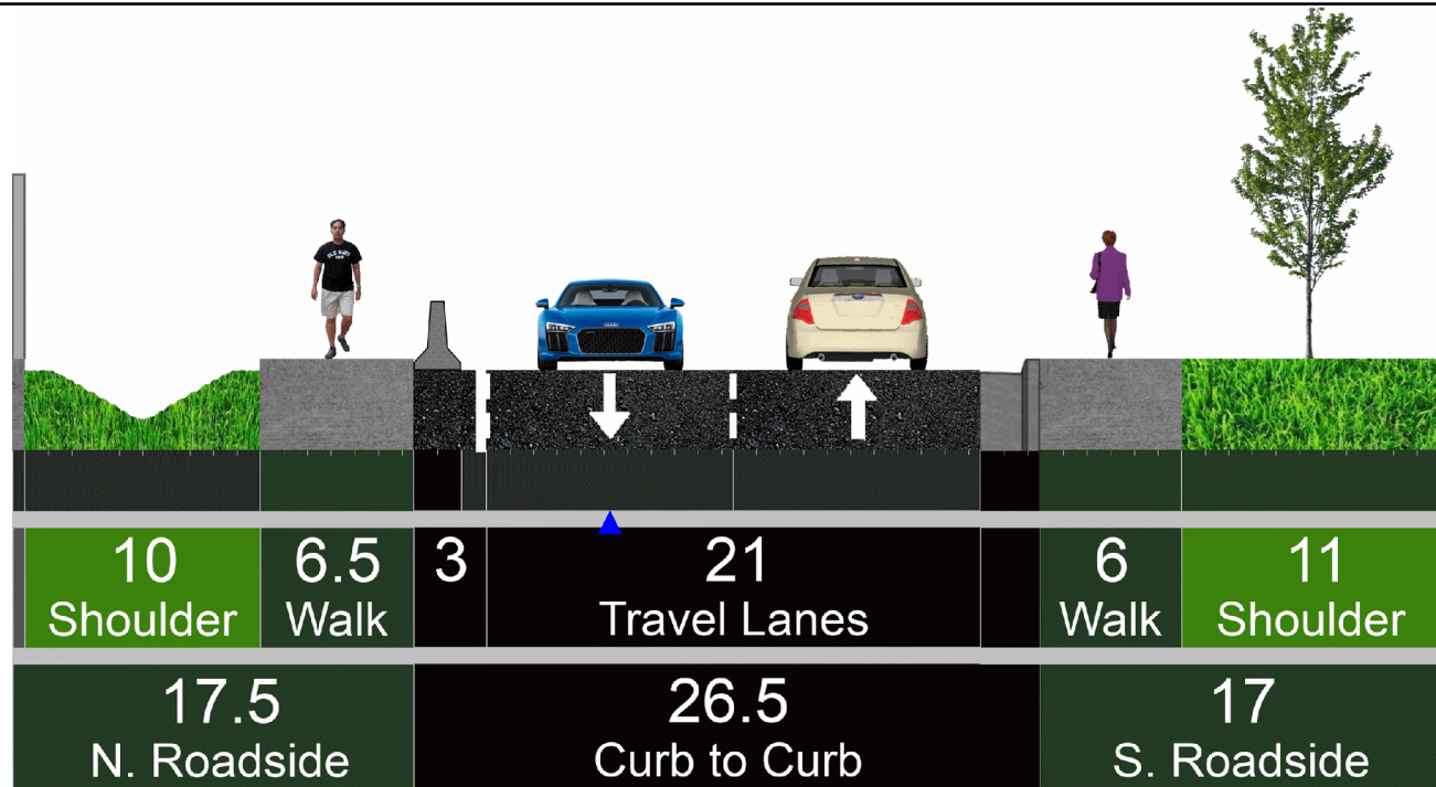
Existing Steele St to Madison Ct Cross Section
