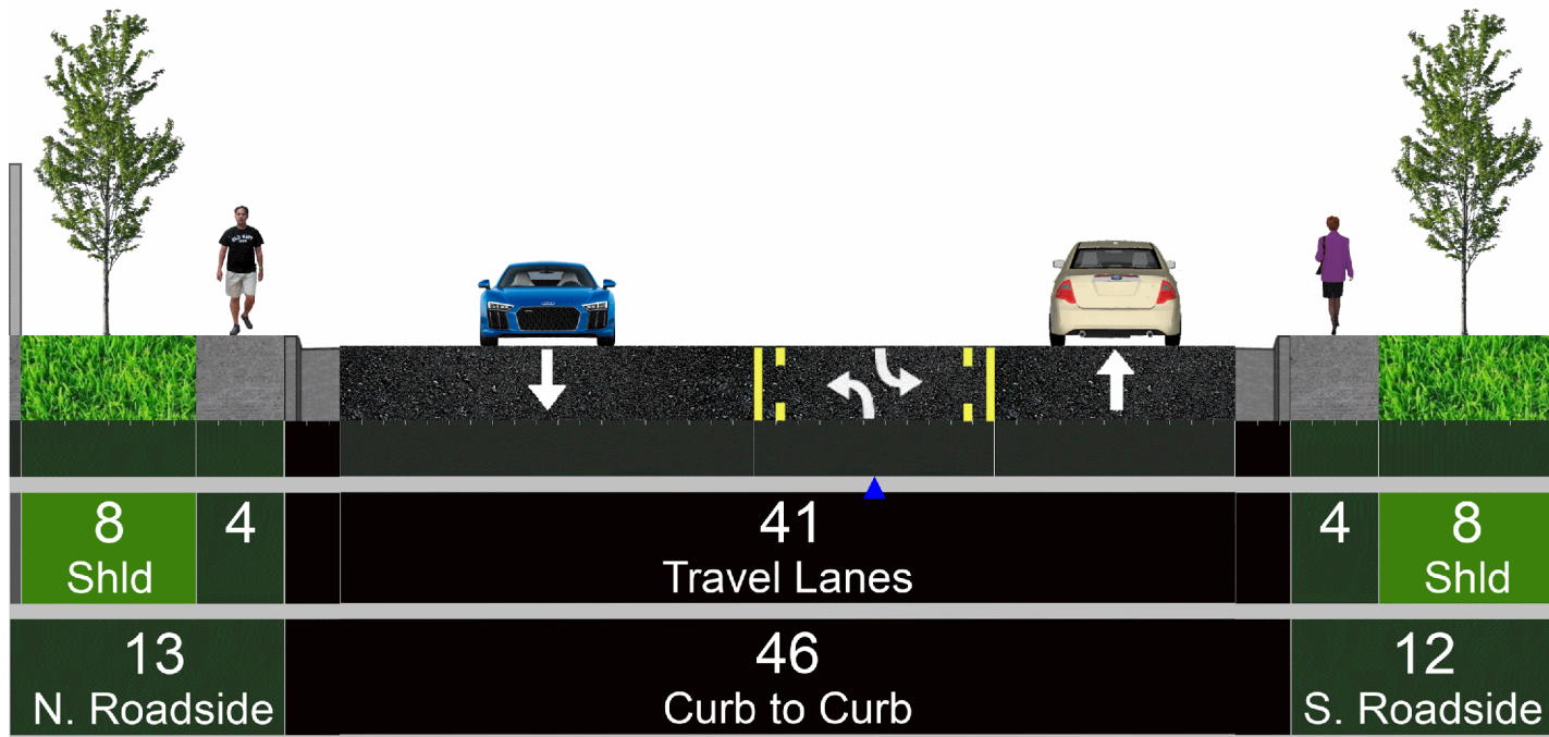
Existing York St to Josephine St Cross Section (Widens at York Street to Create Westbound Right Turn Lane)
