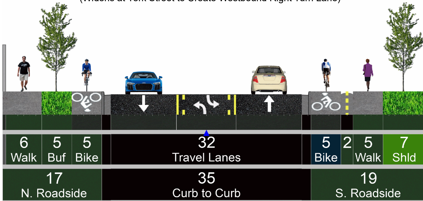
Proposed York St to Josephine St Cross Section
